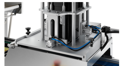
Integrated tray denester
